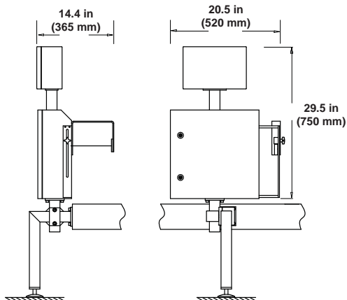
CENTRO FLEX 6 Inch
